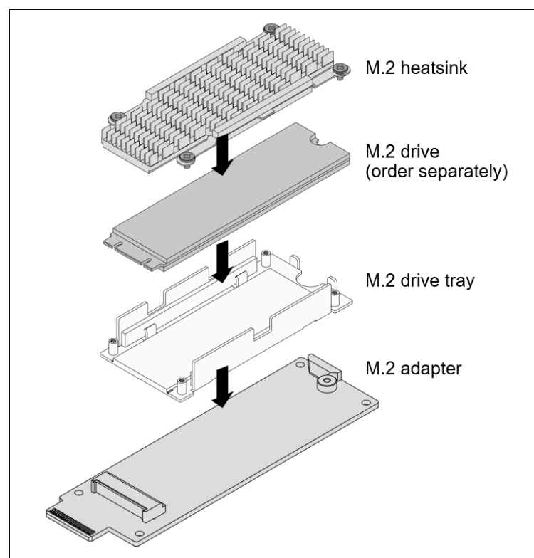
Figure 16. Components of the ThinkSystem V4 Hot Swap M.2 SATA/NVMe Drive Assembly Kit
