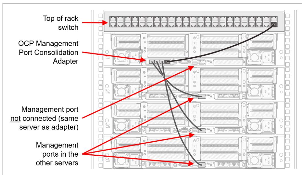
Figure 29. Connections to the ThinkSystem OCP 4 to 1 Management Port Consolidation Adapter
