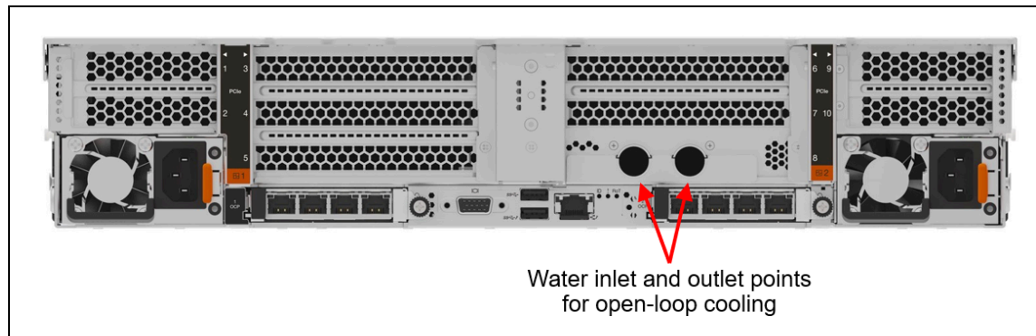
Figure 5. Rear of the SR650a V4 with open-loop water cooling
