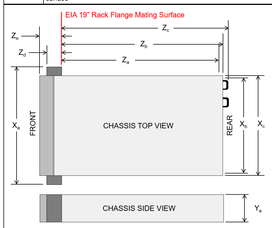
Figure 30. Server dimensions
