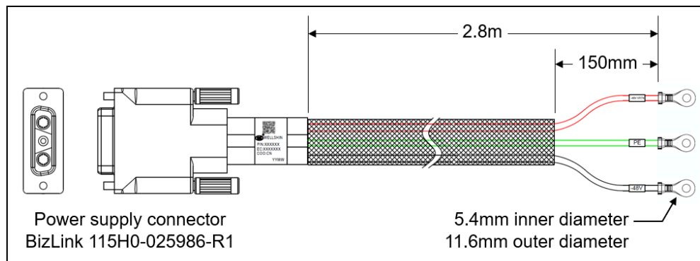
Figure 24. -48V DC power cord
