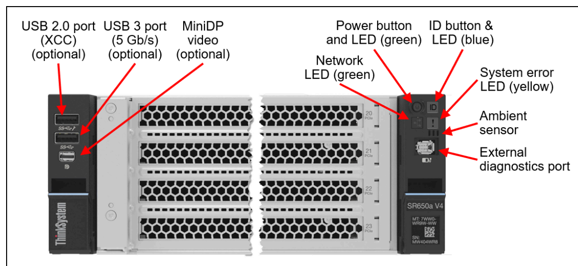
Figure 27. Front operator controls are on the left and right side of the server
