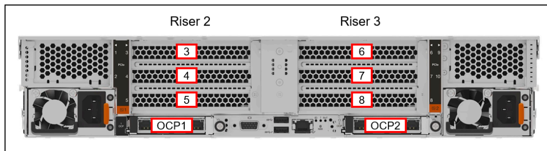
Figure 18. SR650a V4 rear slots
