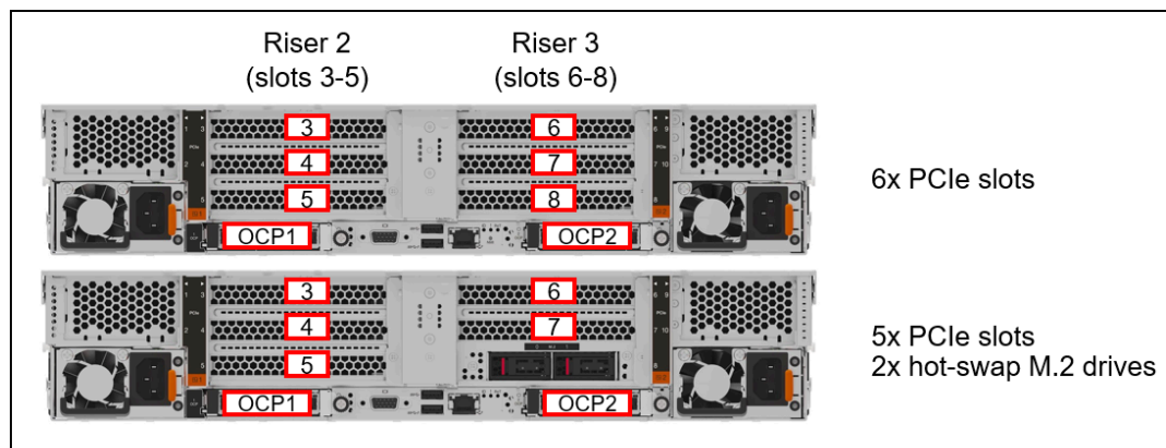
Figure 19. PCIe slot combinations
