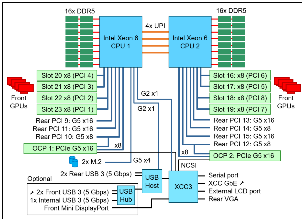
Figure 7. SR650a V4 system architectural block diagram
