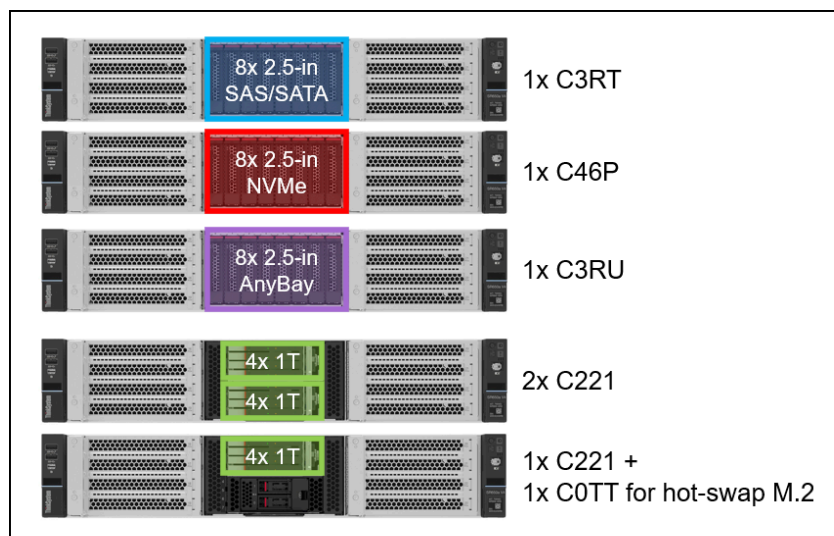
Figure 11. SR650a V4 front drive bay configurations
