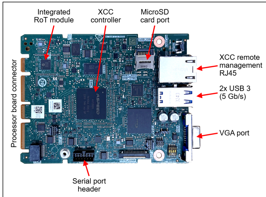
Figure 26. System I/O Board
