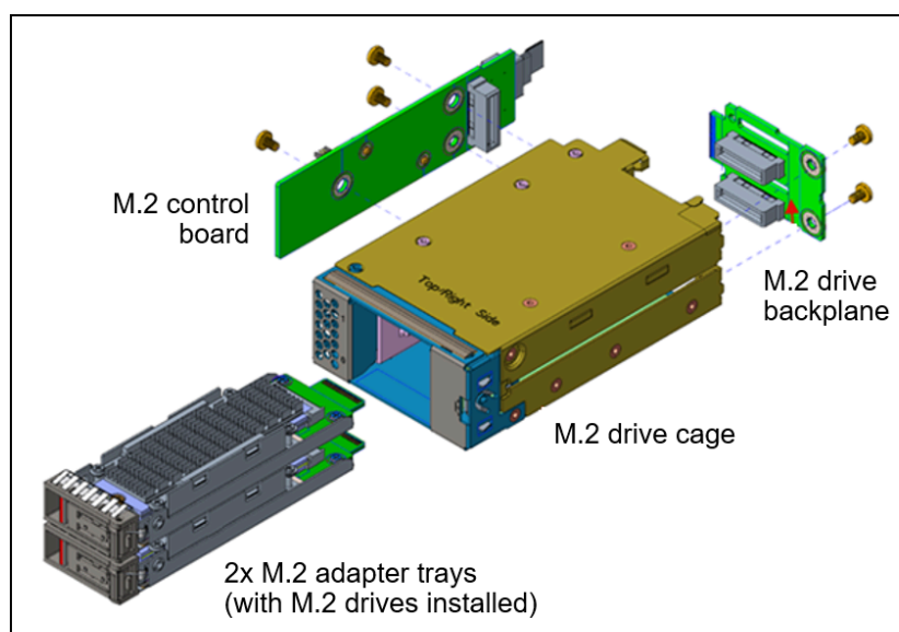
Figure 15. Front hot-swap M.2 drive bays
