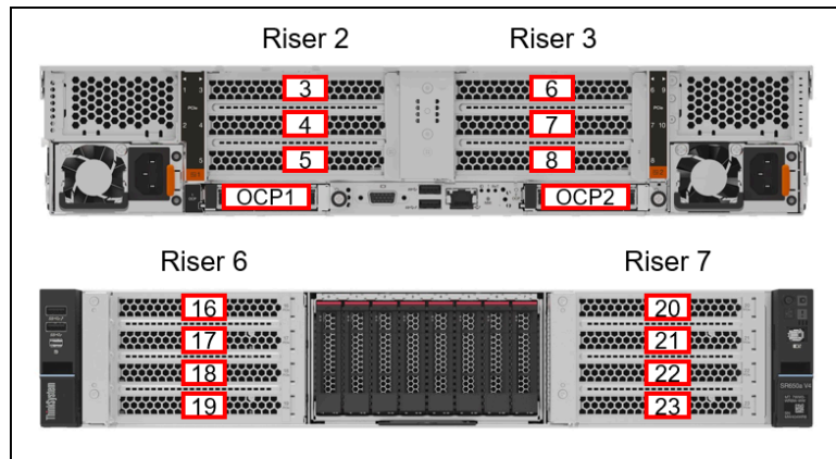
Figure 22. SR650a V4 rear and front slots
