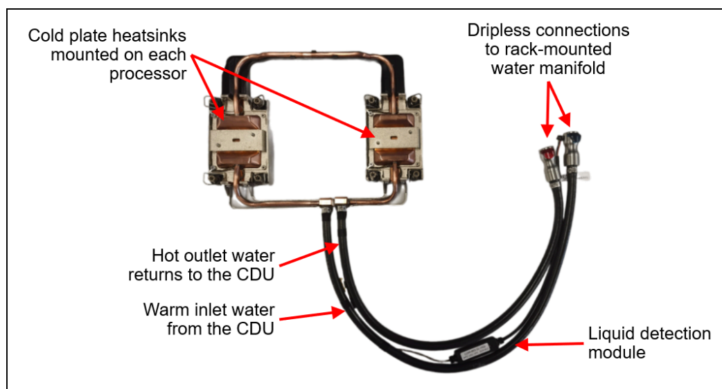
Figure 10. Lenovo Processor Neptune Core Module
