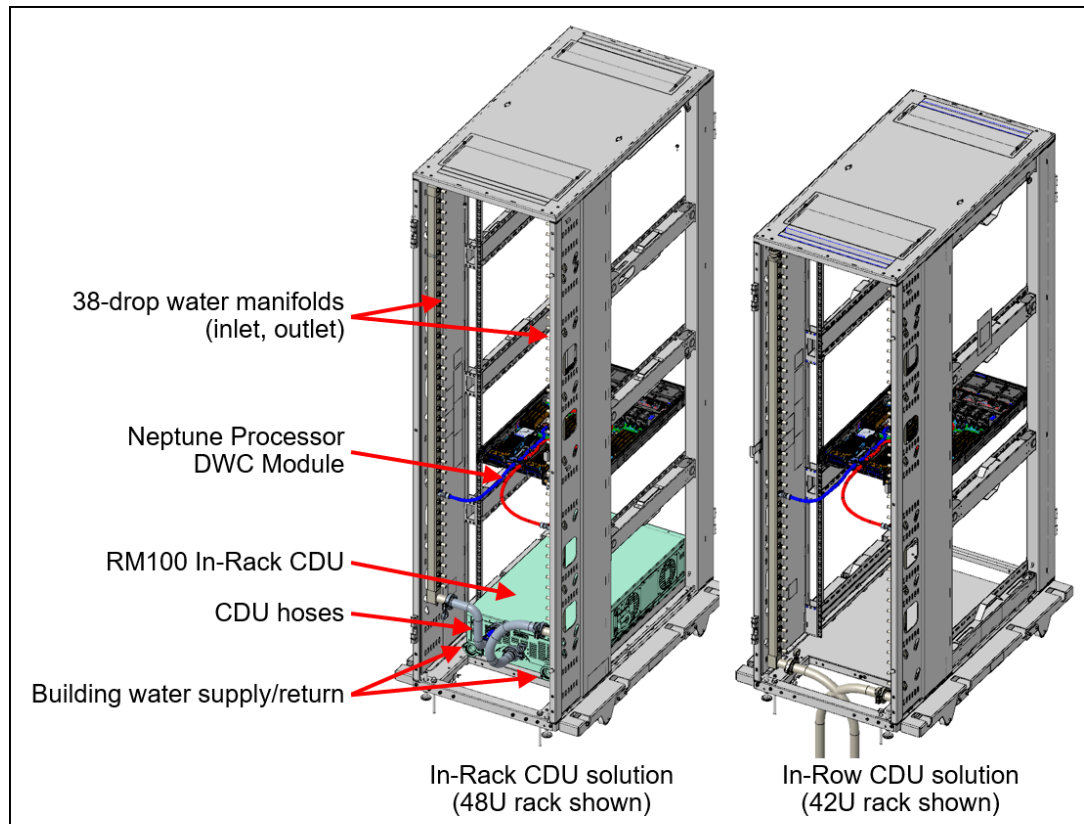
Figure 31. Water manifold connections
