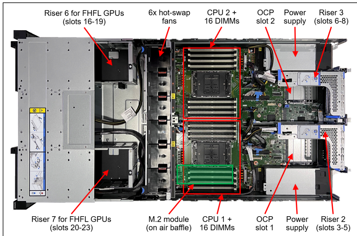
Figure 6. Internal view of the ThinkSystem SR650a V4
