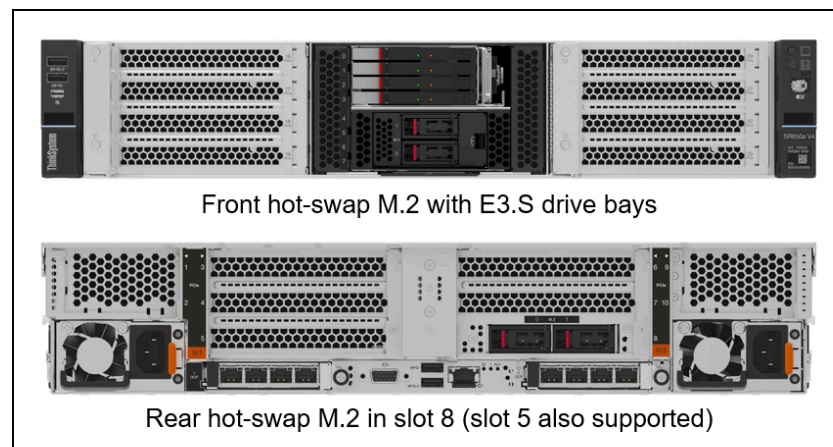
Figure 13. Hot-swap M.2 drive bays
