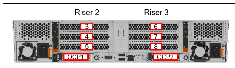
Figure 21. SR650a V4 rear slots
