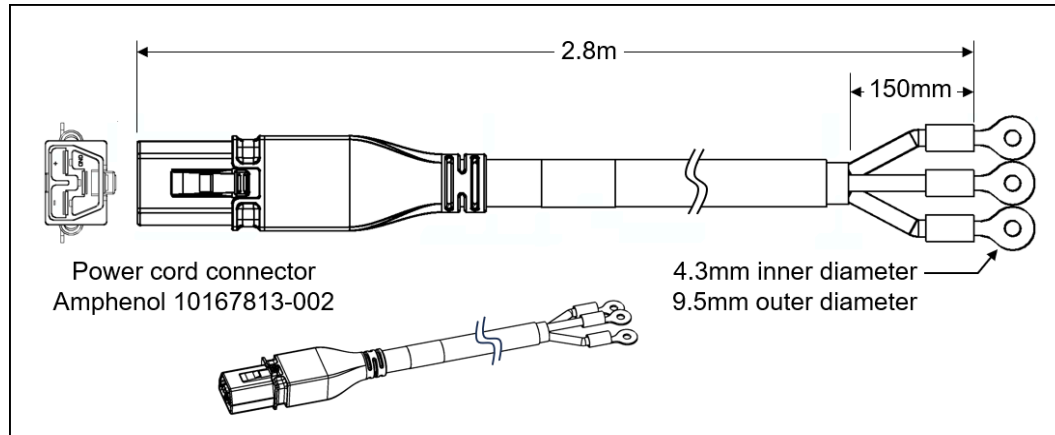
Figure 25. HVDC power cord
