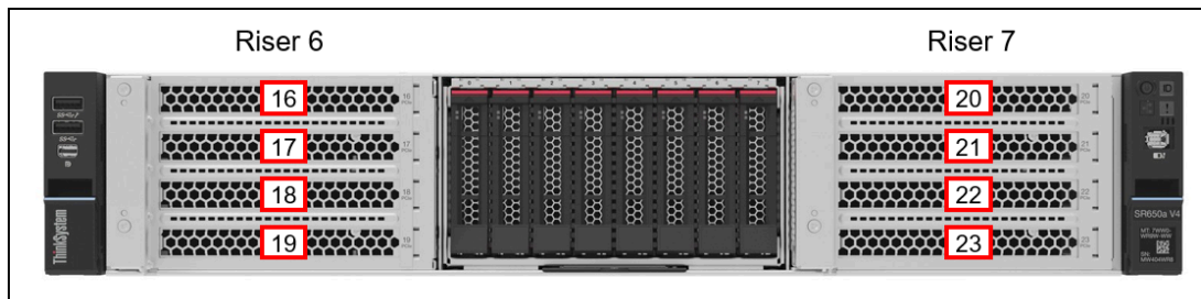
Figure 17. SR650a V4 front slots
